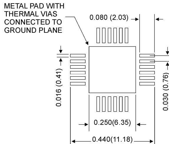
Figure 2. Footprint dimensions shown in inches (mm).
