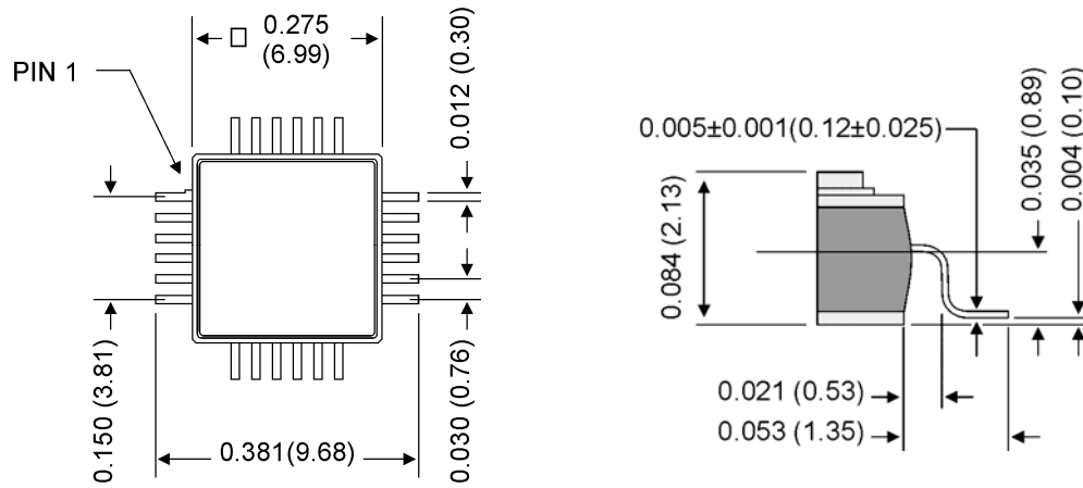
Figure 1. Package outline, dimensions in inches (mm), tolerance \pm 0.002'' ( \pm 0.051\text{mm} ).
