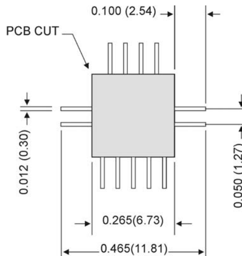
Figure 2. Footprint dimensions shown in inches (mm).
