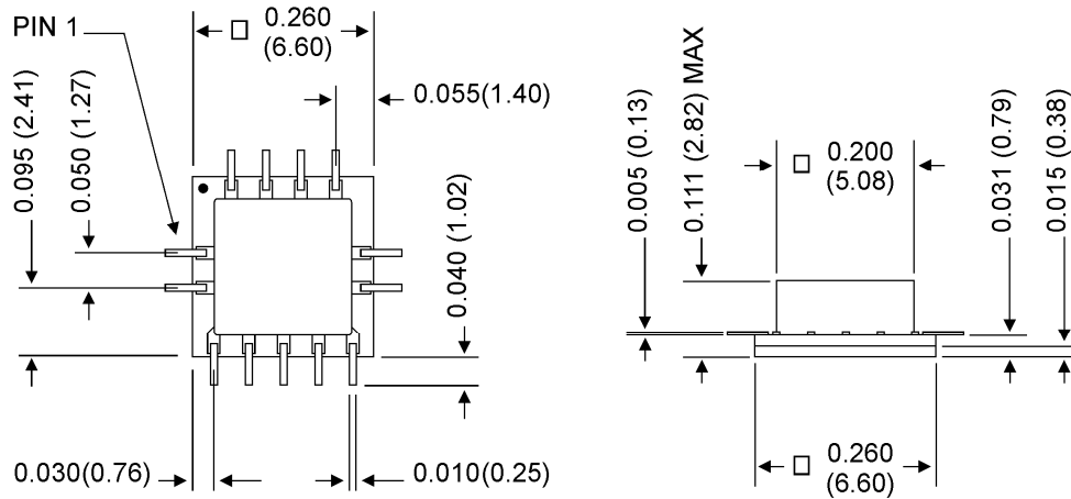
Figure 1. Package outline, dimensions in inches (mm), tolerance \pm 0.003 " ( \pm 0.072 mm).
