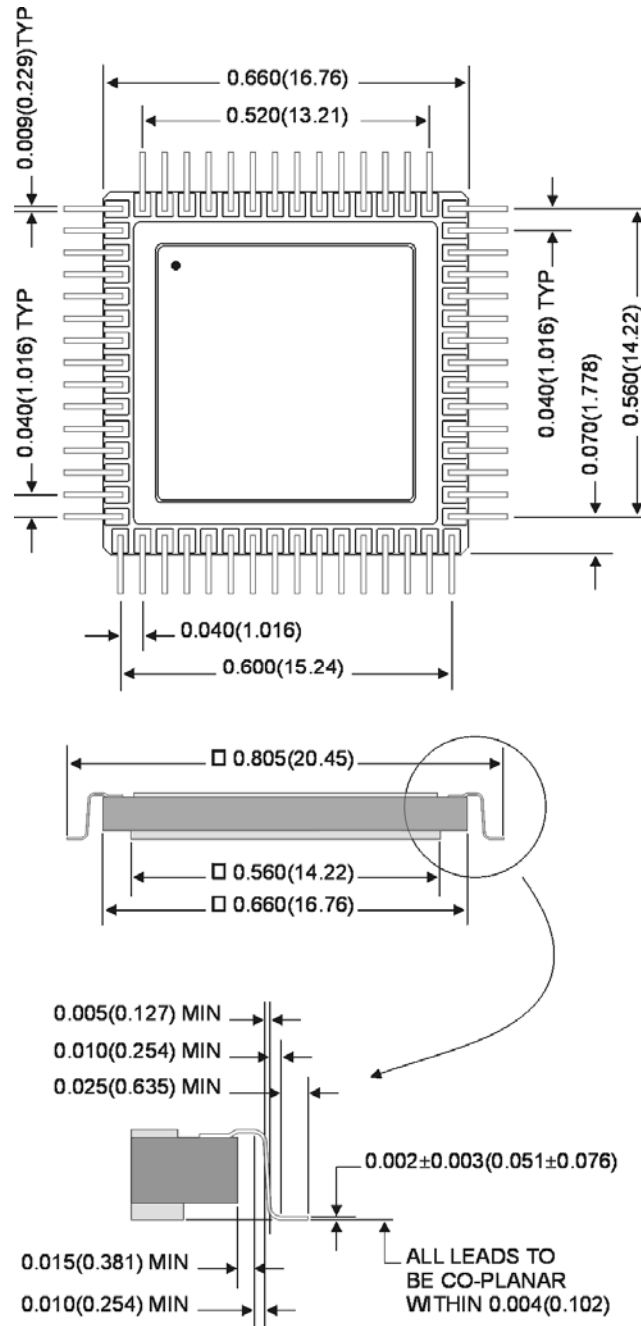
Figure 1. 60 lead QFP package. Dimensions shown in inches (mm).
