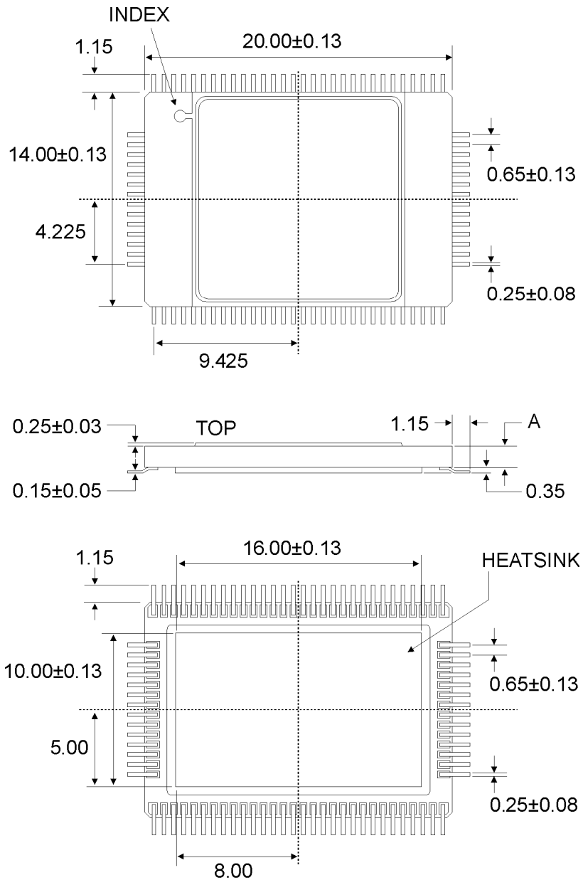
Figure 1. 88 lead QFP package, dimensions shown in mm.
