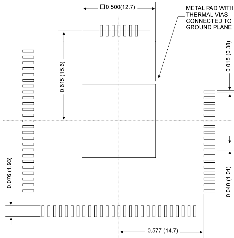
Figure 2. Footprint dimensions shown in inches (mm).
