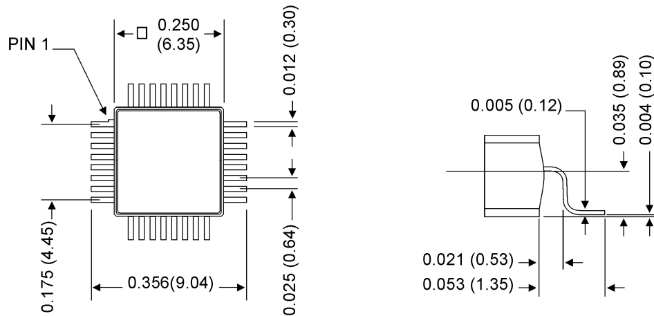
Figure 1. Package outline, dimensions in inches (mm), tolerance \pm 0.002'' ( \pm 0.051\text{mm} ).
