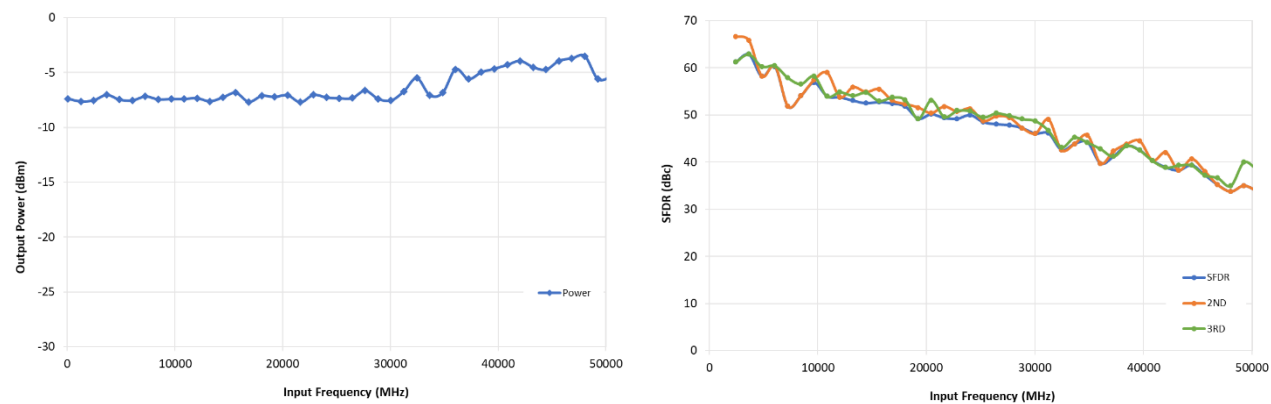
Figure 8 - Input Bandwidth and SFDR for 1.2GHz clock (input at 400mVpp differential).
