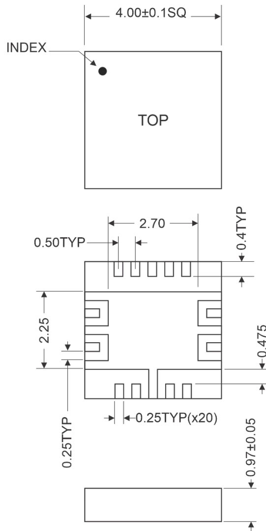
Figure 12 – RTH130-QN package outline, dimensions in mm.
