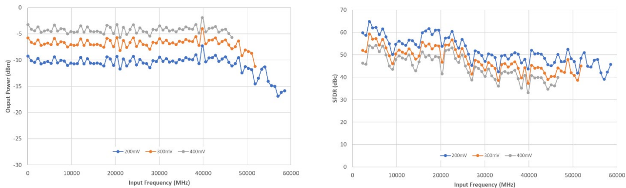
Figure 9 - Input Bandwidth and SFDR for 6GHz clock.
