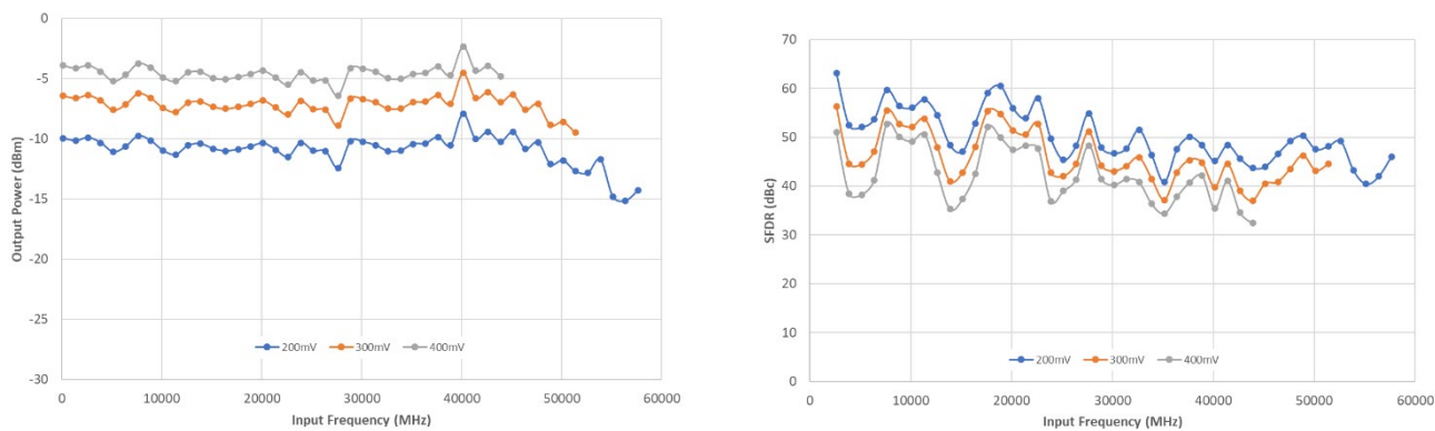
Figure 10 - Input Bandwidth and SFDR for 10GHz clock.
