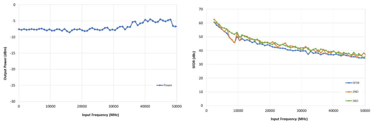
Figure 7 - Input Bandwidth and SFDR for 800MHz clock (input at 400mVpp differential).
