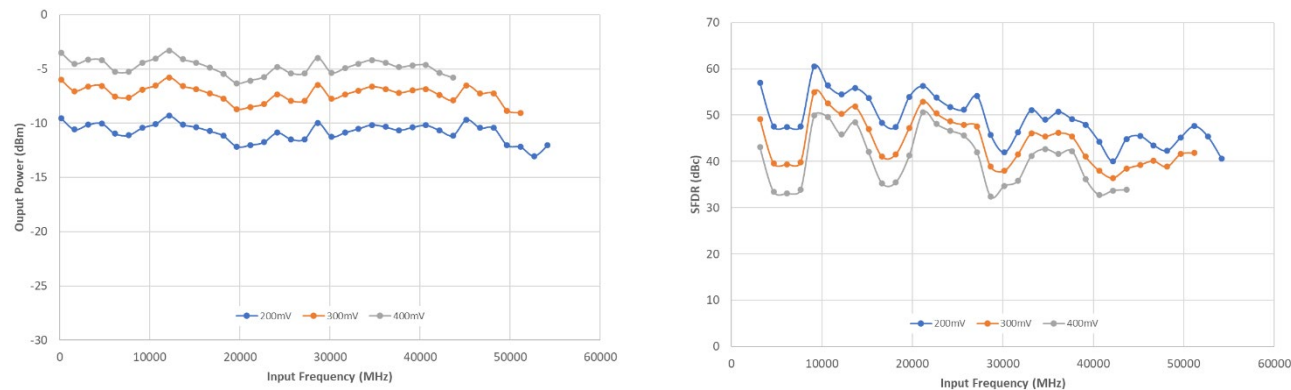
Figure 11 - Input Bandwidth and SFDR for 12GHz clock.
